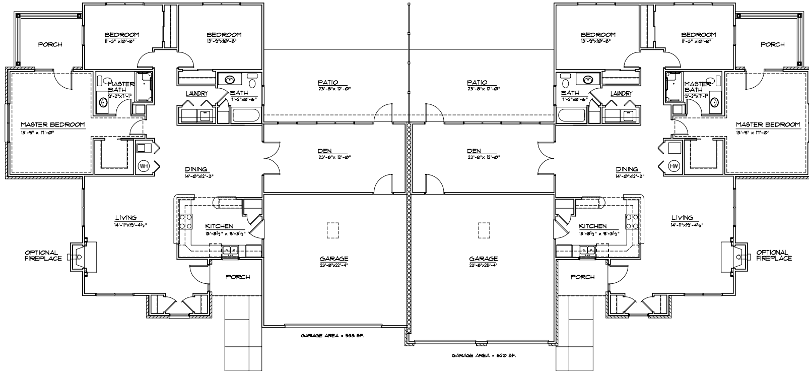
UNIT 'A' - FLOOR PLAN SCALE: 1/4" = 1'-0" (AREA = 1964.2 SF.) (INCLUDING PORCHES AND GARAGE, PATIO AREA NOT INCLUDED.) (AREA = 2651.0 SF.) (PATIO AREA = 286.0 SF.)
